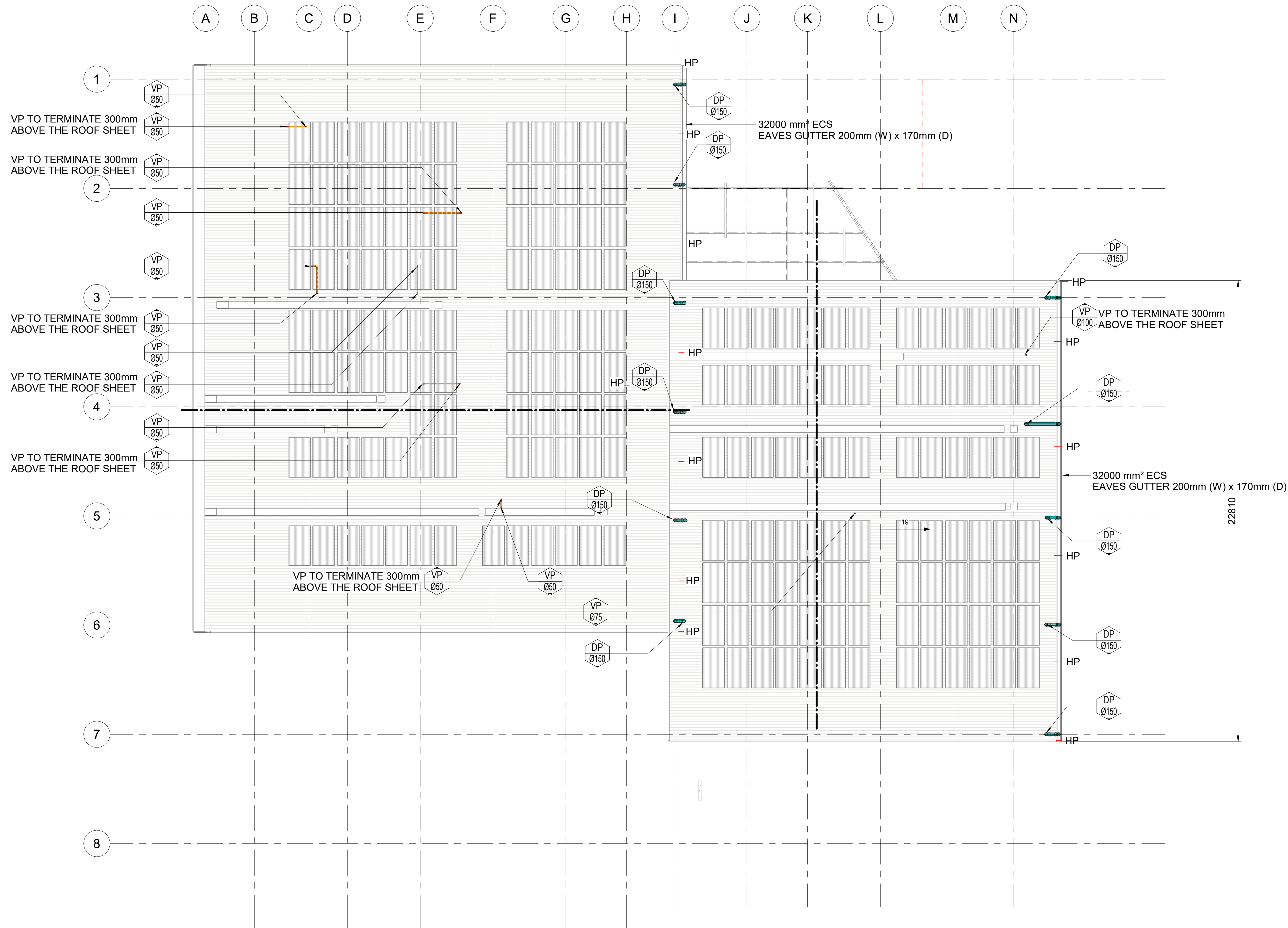
ROOF LEVEL STORM WATER LAYOUT SCALE 1 : 100
